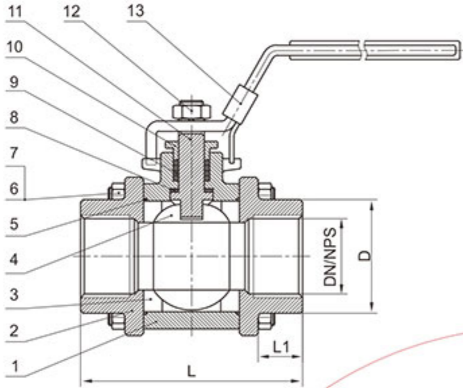
三片式陶瓷球阀 3-PC Ceramic Ball Valve
