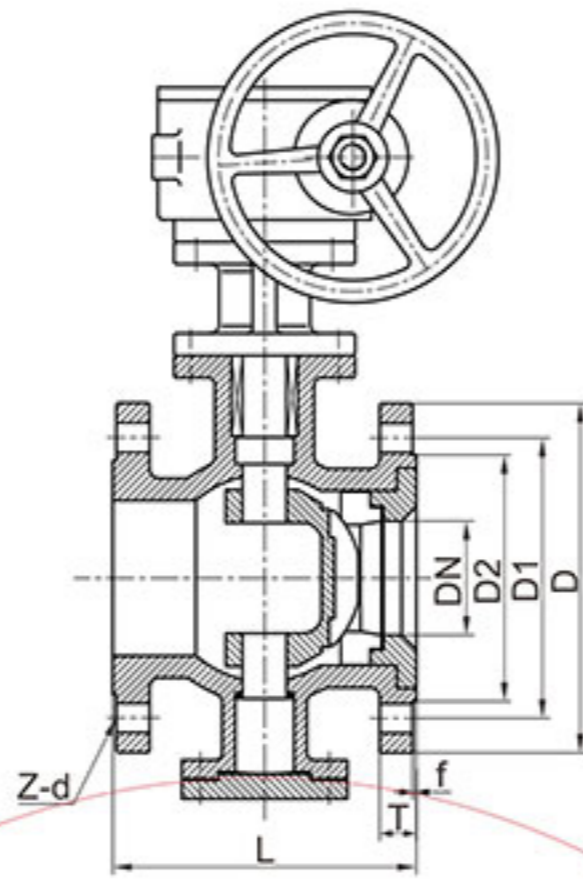
陶瓷偏心半球阀 Ceraminc Eccentric Semi-Ball Valve
