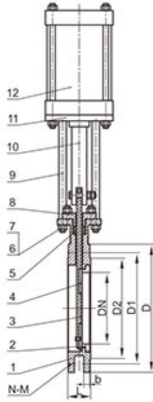
气动薄型陶瓷刀闸阀 Pneumatic Ceramic Knife Gate Valve
